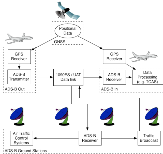
Figure 1: Overview of the ADS-B system architecture. Aircraft receive positional data that is transmitted via the ADS-B Out subsystem over the 1090ES or the UAT data link. It is then received and processed by ground stations and by other aircraft via the ADS-B In subsystem.
