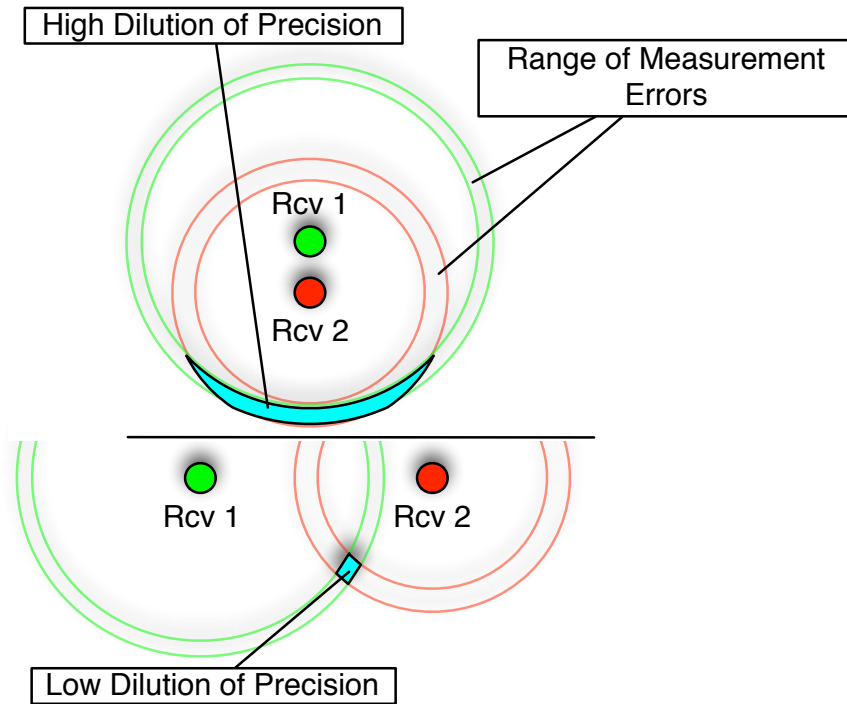
Figure 3: Geometric dilution of precision. The circles show the measurement errors of the respective receivers; the intersections demonstrate the area where the true location of the measured object can be found. An adverse placement of receivers in relation to the target (top) can severely affect the outcome of the localization compared to a favorable deployment (bottom).
