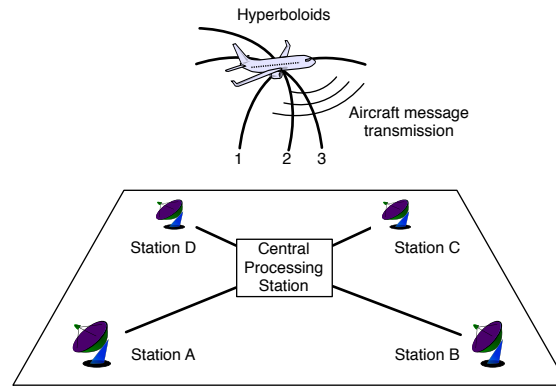
Figure 2: Basic multilateration architecture with four receivers and three resulting hyperboloids.
