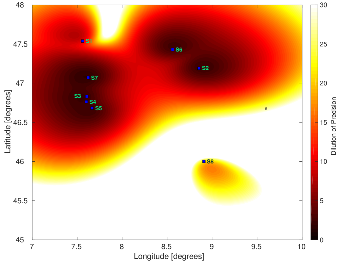
Figure 4: The map shows the geometric dilution of precision of our 8 sensor measurement system for wide area multilateration. All sensors are on the ground, the assumed measurement altitude is 38,000 feet.
