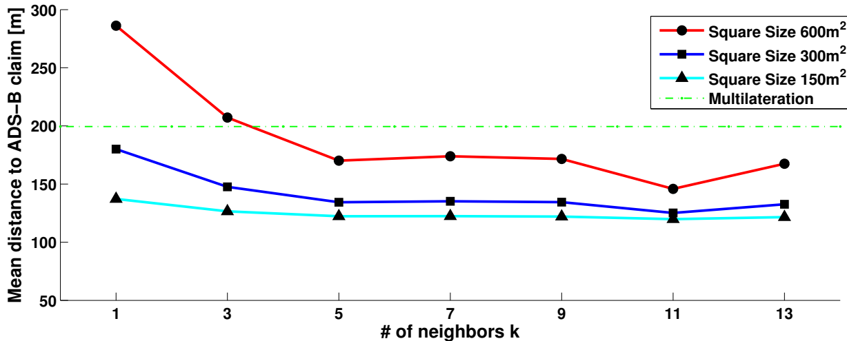
Figure 7: Optimal choice of neighbors k for different square sizes (MLAT as comparison).
