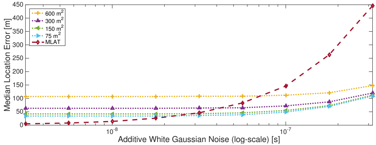
Figure 8: Median location error depending on the level of noise N affecting the measurements. k-NN results obtained with k = 5 and 4 different square sizes.
