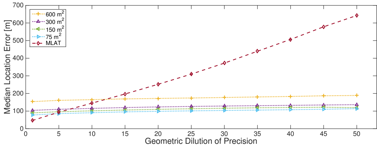
Figure 9: Median location error depending on the geometric dilution of precision affecting the measurements at a noise level of N = 10^{-7} s . k-NN results obtained with k = 5 and 4 different square sizes.
